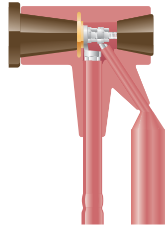
Straight adapter for vertical connection of the termination to SF 6 -insulated switchgear
