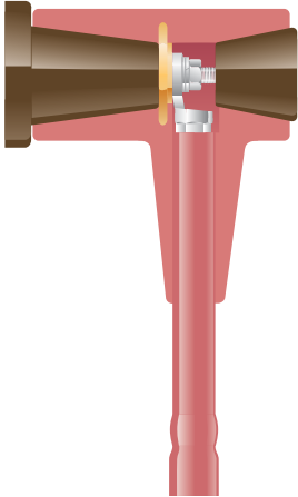
T-adapter for perpendicular connection of the termination to SF 6 -insulated switchgear
