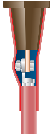
T-adapter for perpendicular connection of termination and surge arrester to SF 6 -insulated switchgear
