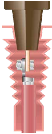
Raychem right angle or inline application RCAB up to 17.5 kV
